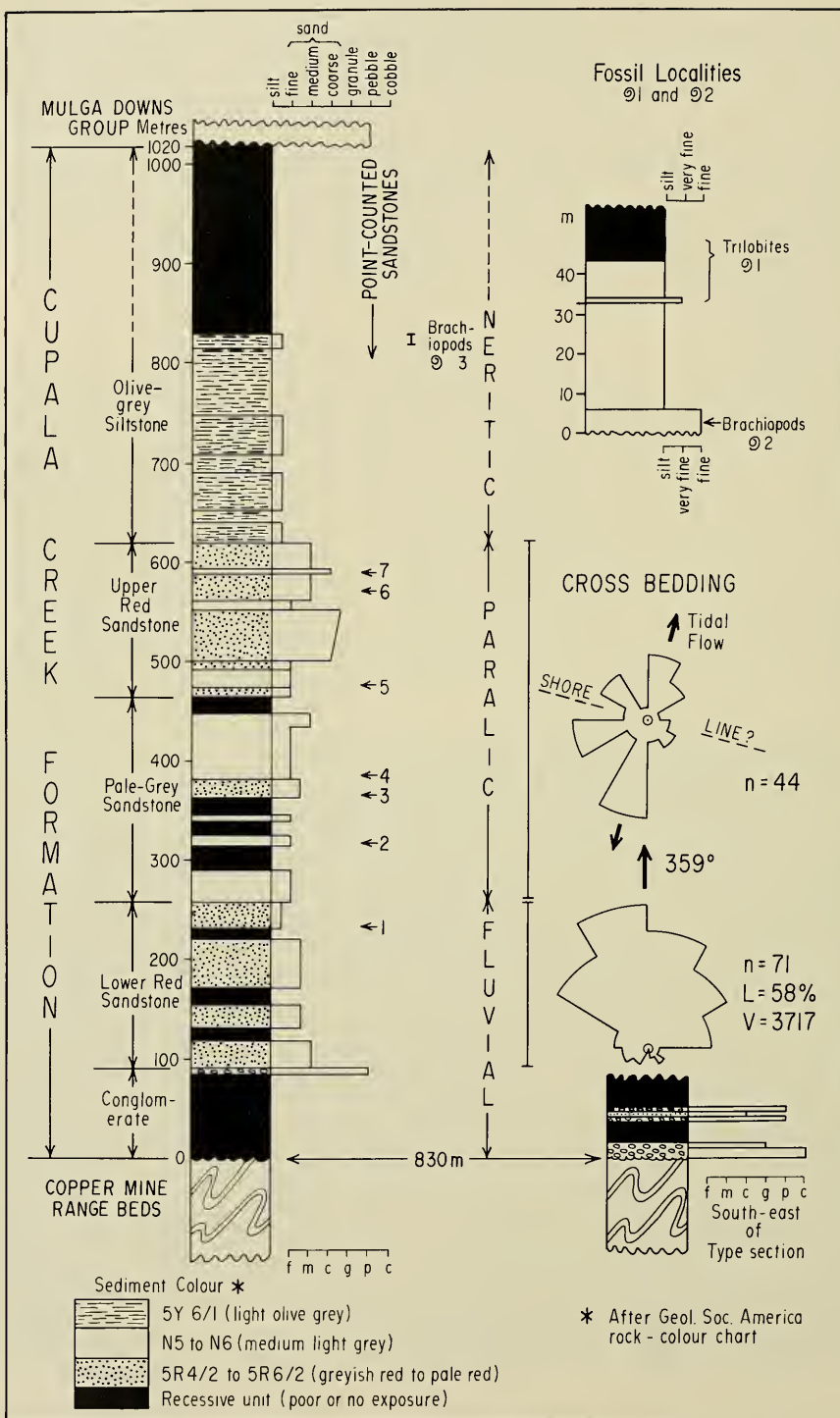
Fig. 3. Type section of the Cupala Creek Formation.
